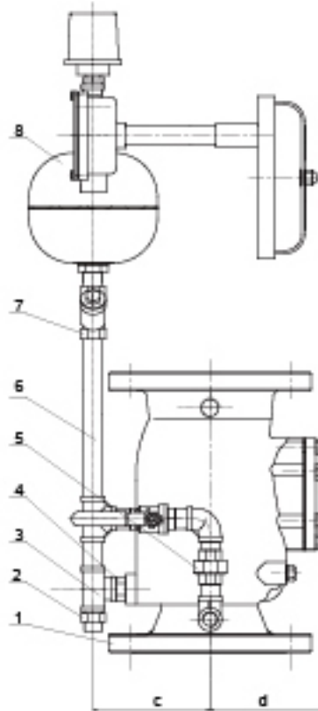
ASSEMBLY DRAWING WITHOUT COMPENSATOR SYSTEM
