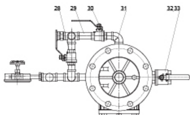
ASSEMBLY DRAWING WITHOUT COMPENSATOR SYSTEM
